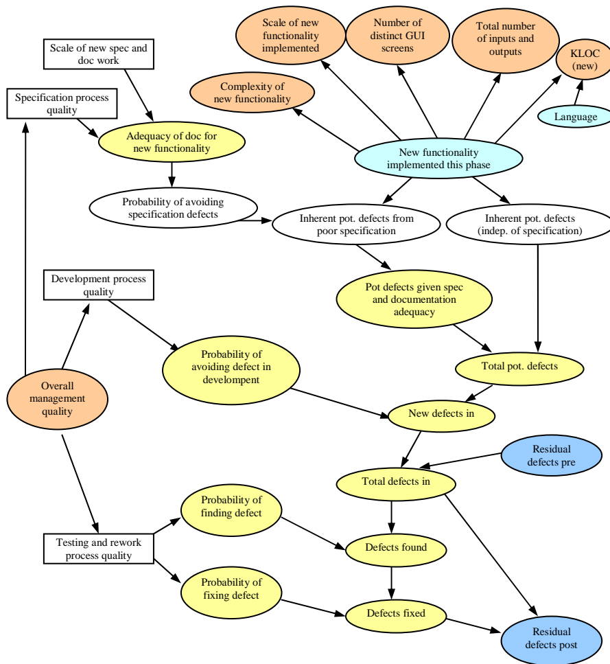
Fig. 1. Schematic view of phase-based defect prediction model; adopted from [2, 3]
